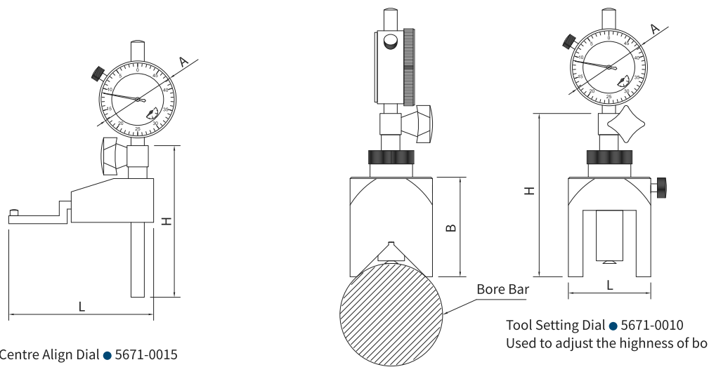
Dial Bore Gauge ● 5671-0005 Used to measure cylinder bore without unloading bore
