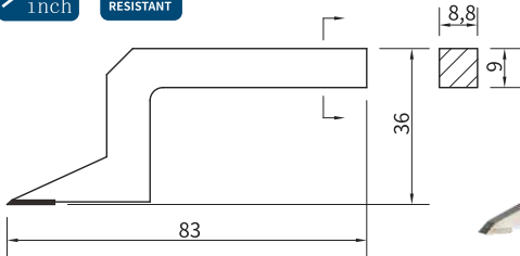
3130-4103 For:3130-4703 Range:0-300/0-12" 3130-4103 For:3130-4716 Range:0-600/0-24" 3130-4103 For:3230-4705 Range:0-300/0-12" 3130-4103 For:3230-4710 Range:0-600/0-24"
